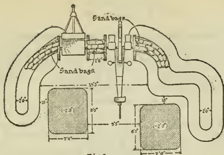
Fig. 1. Easiy entrenchment for field artillery. Protection against rifle fire and shrapnel
